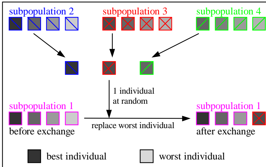
Fig. 8-5: Scheme for migration of individuals between subpopulation
