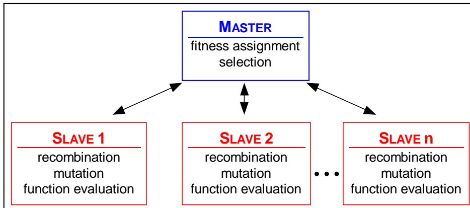
Fig. 8-2: Global population model (master-slave-structure)
