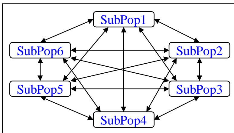
Fig. 8-4: Unrestricted migration topology (Complete net topology)
