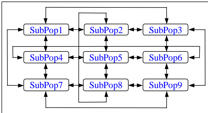
Fig. 8-7: Neighborhood migration topology (2-D grid)
