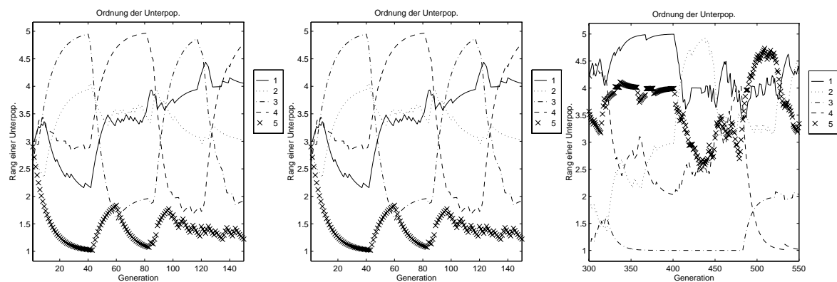
Fig. 9-2. Application of different strategies, order of subpopulations; left: beginning of optimization run, middle: middle phase, right: final phase
