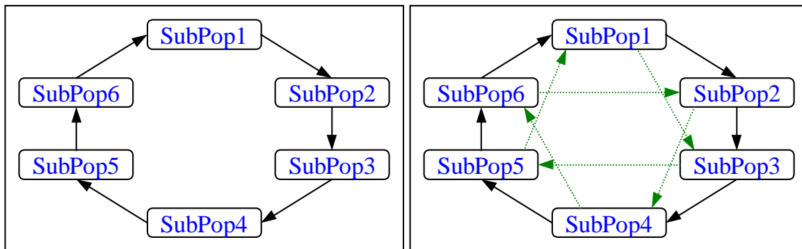
Fig. 8-6: Ring migration topology; left: distance 1, right: distance 1 and 2
