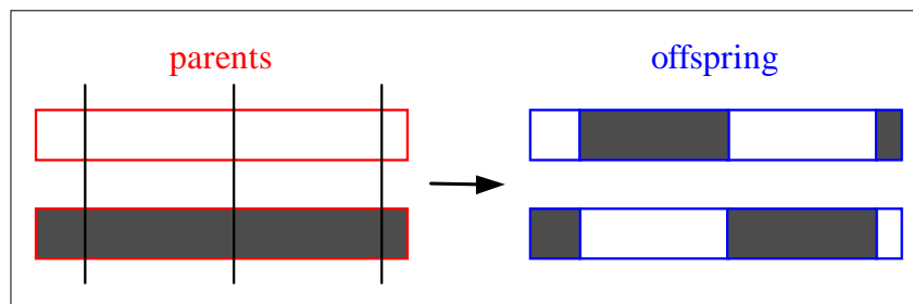
Fig. 4-7: Multi-point crossover
