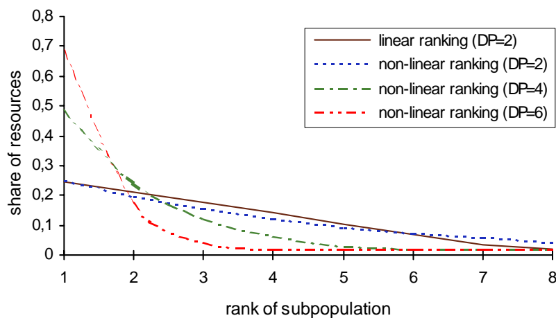
Fig. 9-1. Division of resources for subpopulations: linear and non-linear ranking and different values of division pressure
