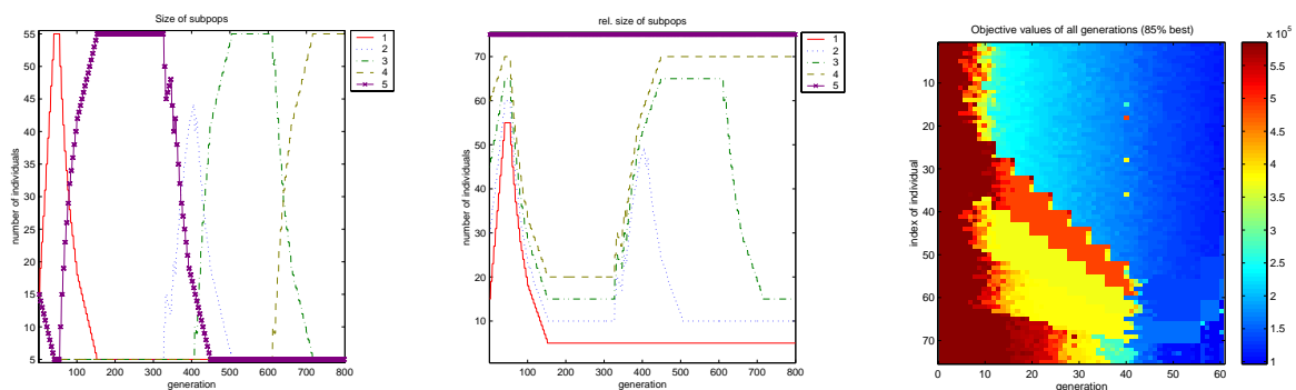
Fig. 9-3. Competing subpopulations; left: size of subpopulations, middle: relative size of subpopulations, right: objective values of all individuals at the beginning of the optimization run
