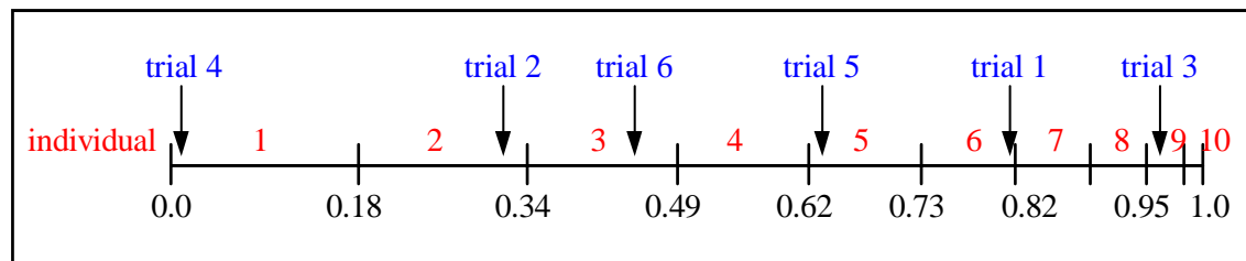
Fig. 3-3: Roulette-wheel selection
